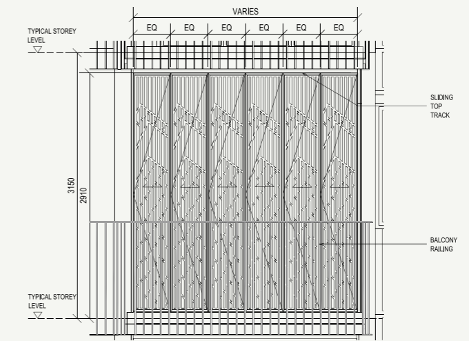
3 BALCONY / PES SCREEN - FRONT ELEVATION (External View)
